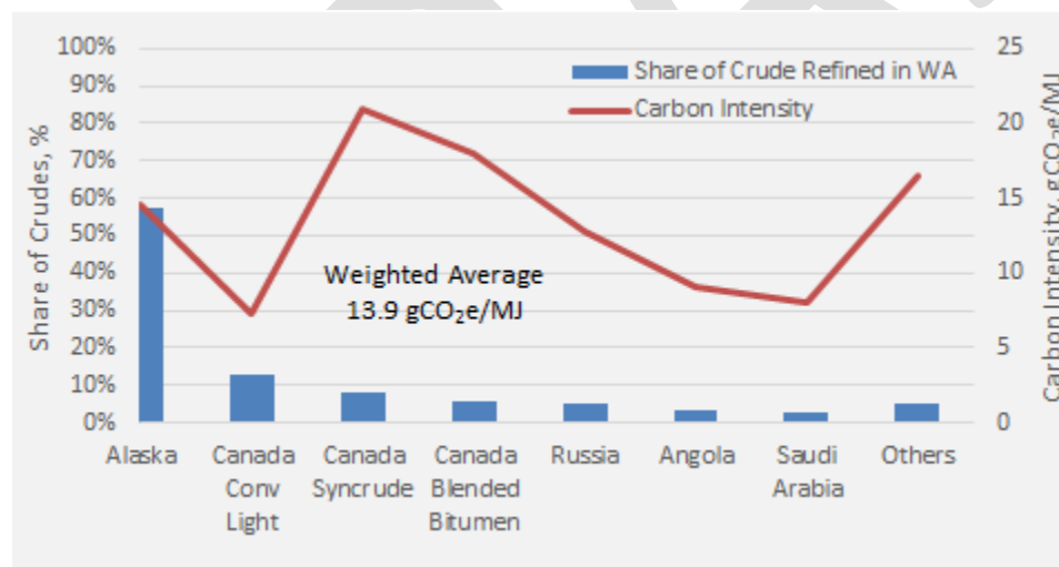
Figure 3-4. Average CI for crude oils refined in Washington.
