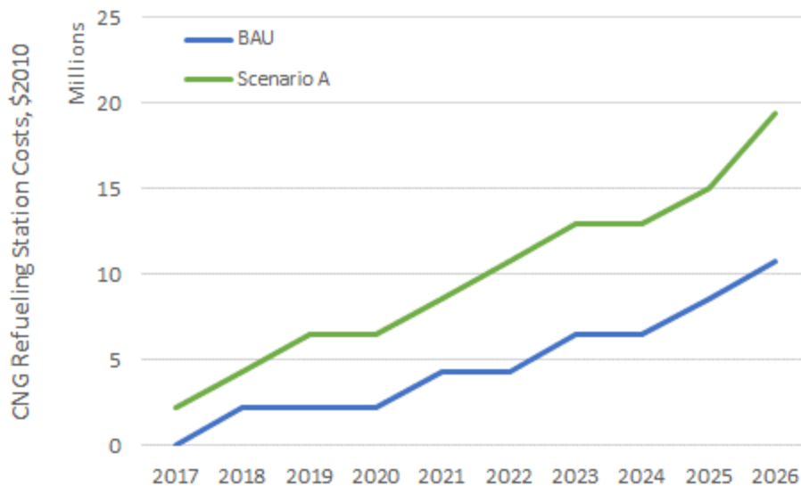
Figure 5-32. Projected cumulative CNG refueling infrastructure spending.
