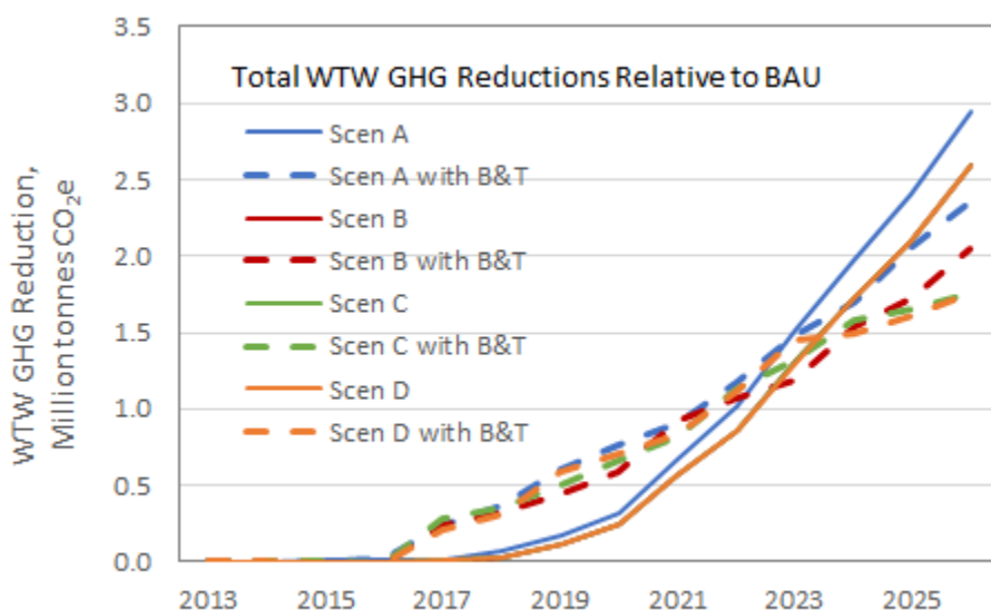
Figure 5-24. WTW GHG Emission Reductions Relative to BAU
