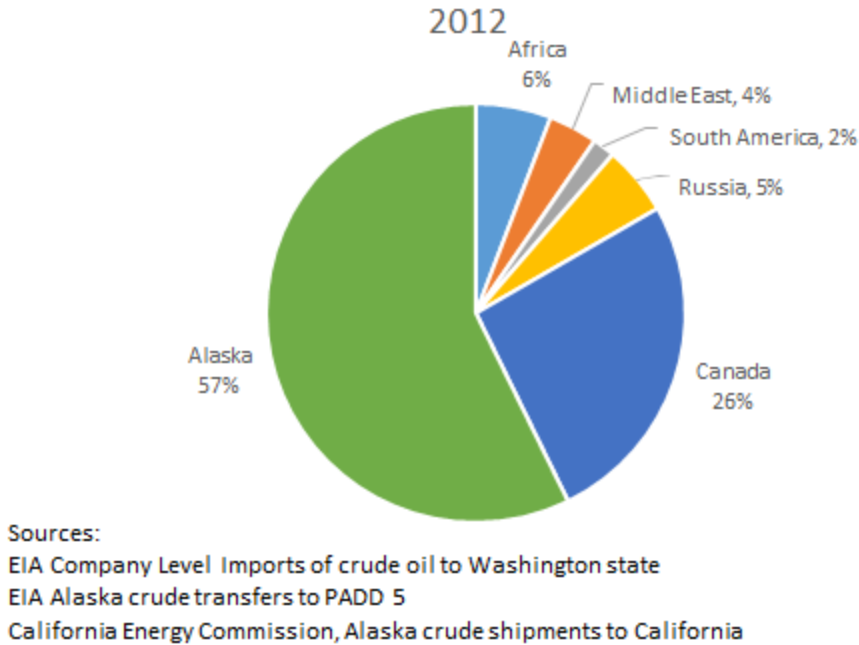
Figure 3-1. Sources of Crude Oil Supplied to Washington State in 2012 by Region.
