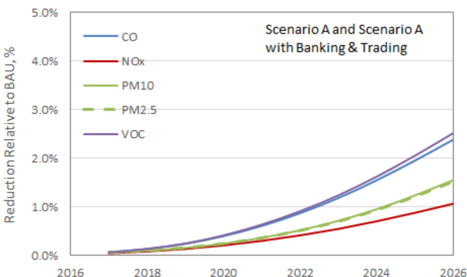
Figure 5-25. Emission reductions relative to BAU for both versions of Scenario A.
