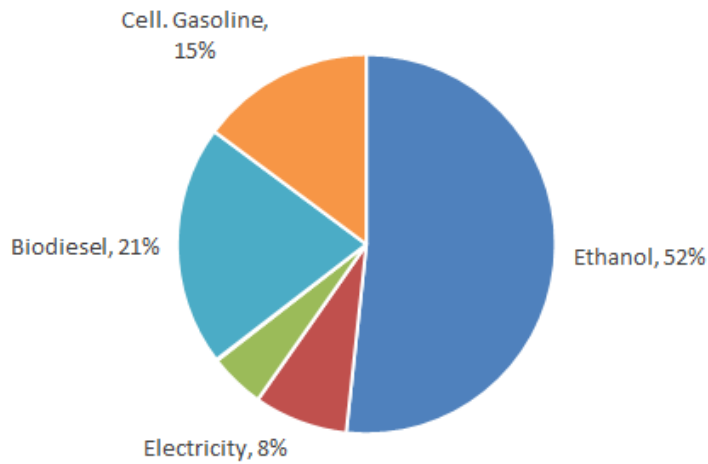
Figure 5-18. Relative contribution to compliance in 2026, Scenario D (low cellulosic E15)
