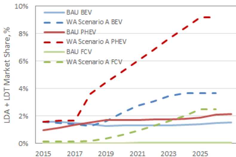
Figure 4-4. Comparison of Scenario A and BAU LDV Market Shares.
