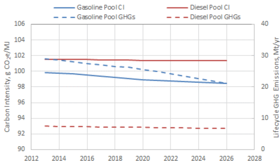
Figure 4-2. BAU Carbon Intensity and Lifecycle GHG Emission Forecasts.
